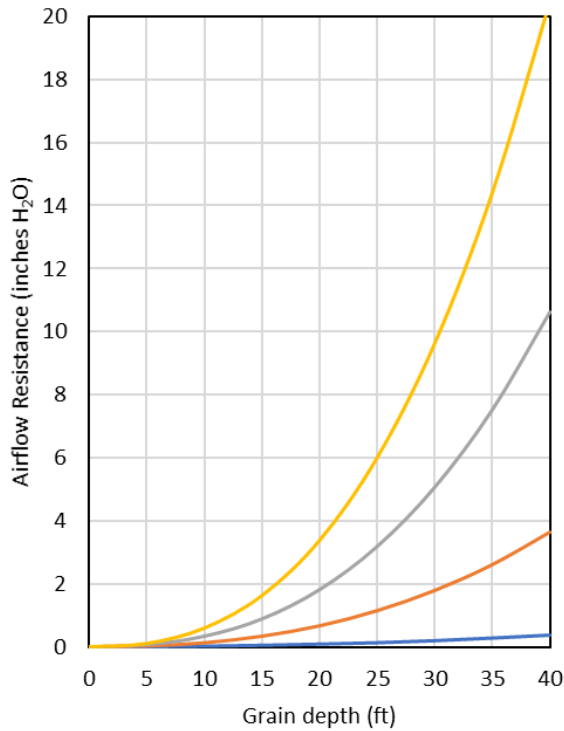
Airflow Resistance of Peas
