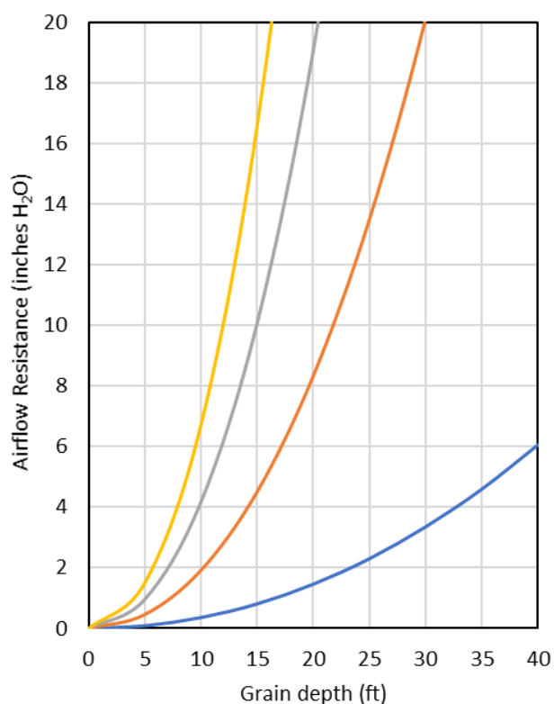
Airflow Resistance of Canola
