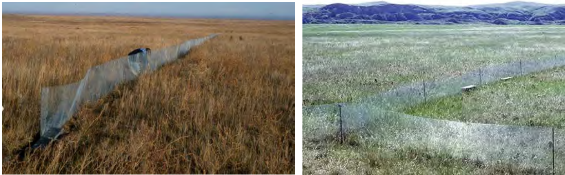
Figure 13: Different Configurations of Barrier Fences and Trap Arrays Constructed of Galvanized Mesh with Snake Funnel Traps
