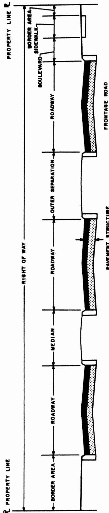
MULTI-LANE DIVIDED HIGHWAY
