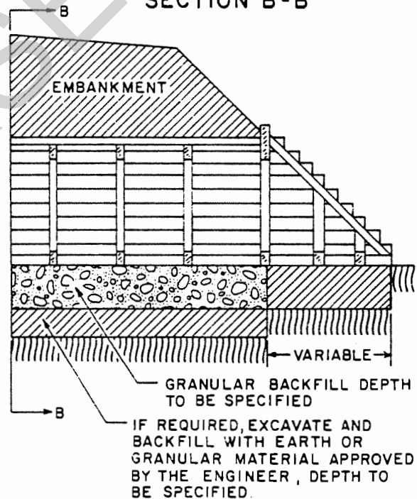
ELEVATION WITH GRANULAR BACKFILL
