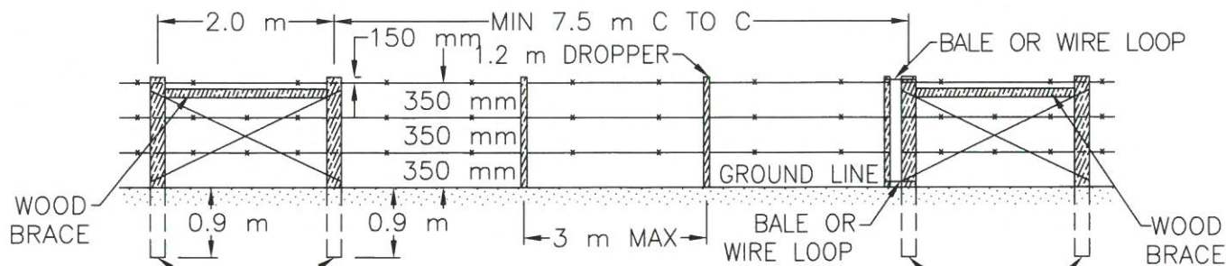
DETAIL OF GATE
