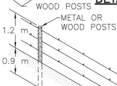
PERSPECTIVE OF FENCE CORNER
