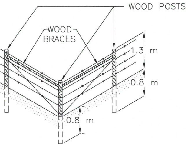
PERSPECTIVE OF FENCE CORNER
