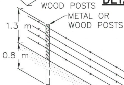
PERSPECTIVE OF FENCE CORNER
