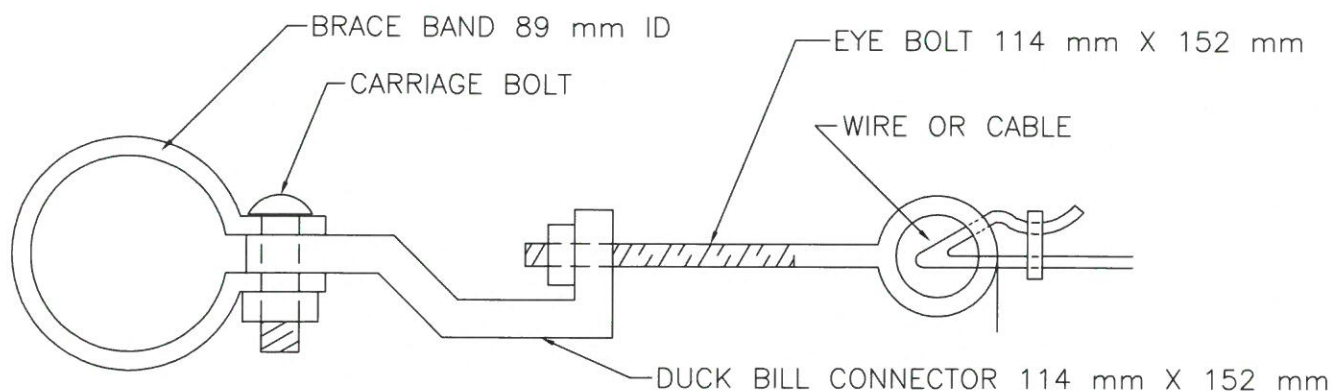
DETAIL 'A' - DUCK BILL ASSEMBLY
