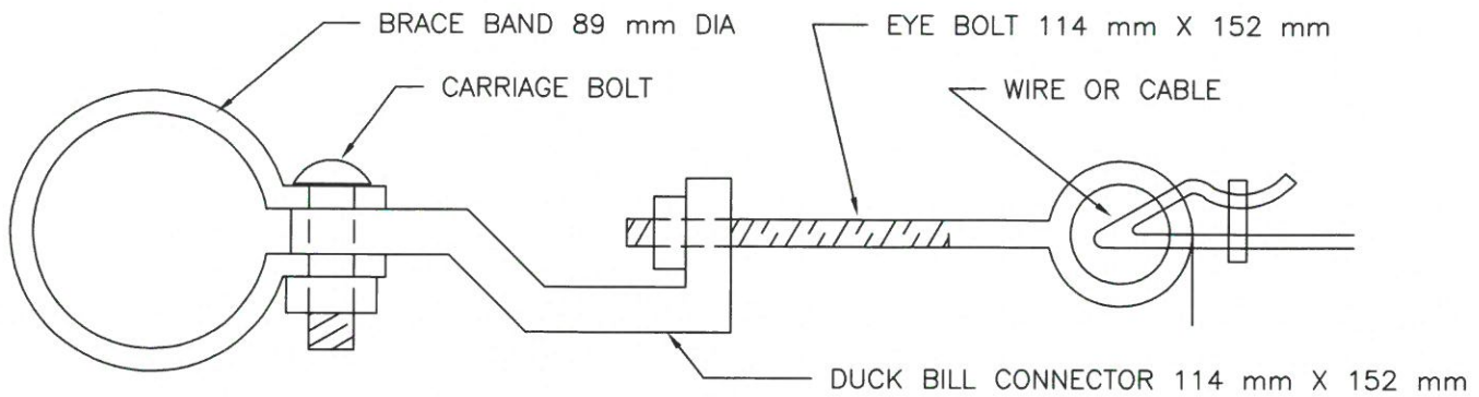
DETAIL 'A' - DUCK BILL ASSEMBLY
