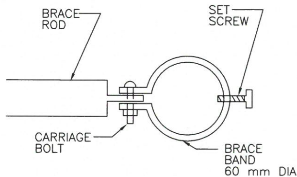
DETAIL 'B' - BRACE BAND
