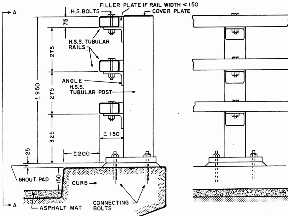
SECTION: RAIL AND POST SCALE: N.T.S.
