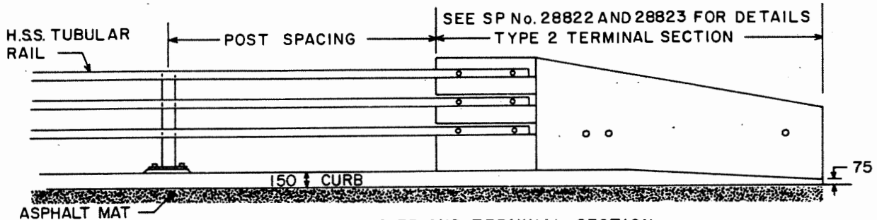
ELEVATION: BARRIER AND TERMINAL SECTION SCALE: N.T.S.
