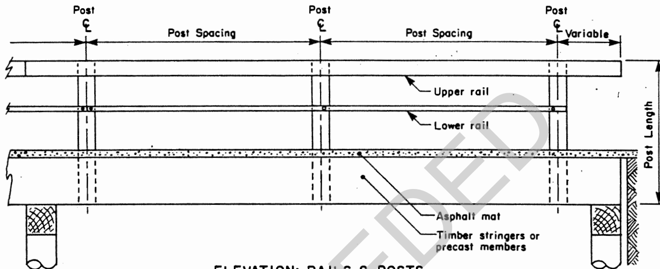
ELEVATION: RAILS & POSTS
