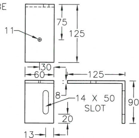
BRACKET DETAIL
