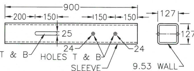
PLAN VIEW: EXPANSION SLEEVE
