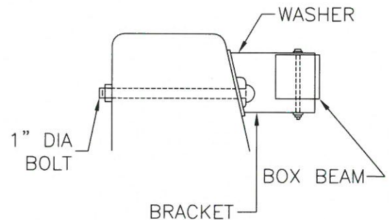
SECTION A-A ATTACHMENT BRACKET
