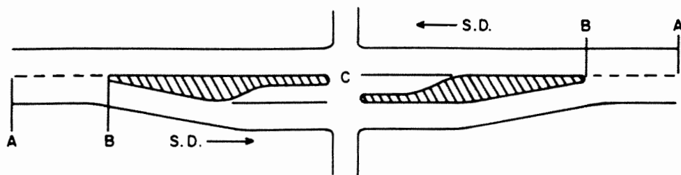
CHANNELIZED INTERSECTION
