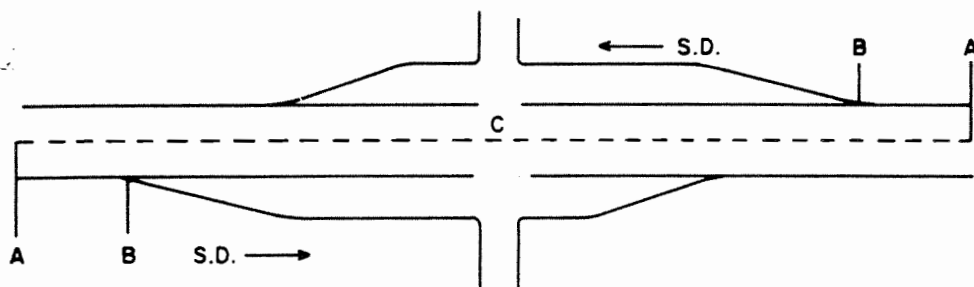
DOUBLE TYPE "A" OR "B" TREATMENT
